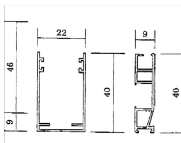
Dimensions – Side guides and bottom bar
