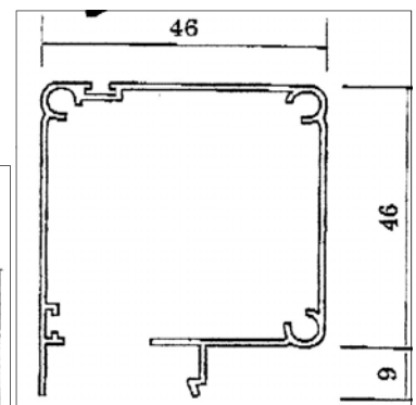
Dimensions – Cassette case
