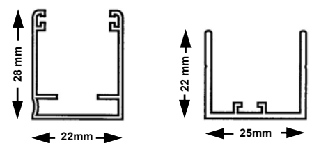
Side Rail
