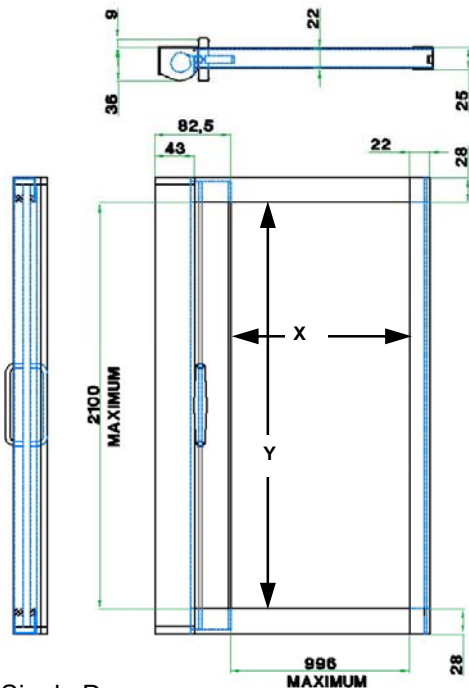
Single Door
